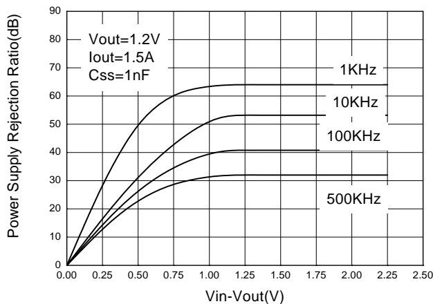
Figure 13 V IN PSRR vs. (V IN -V OUT )
