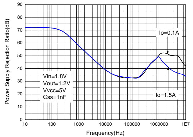
Figure 12 V CC PSRR vs. Frequency
